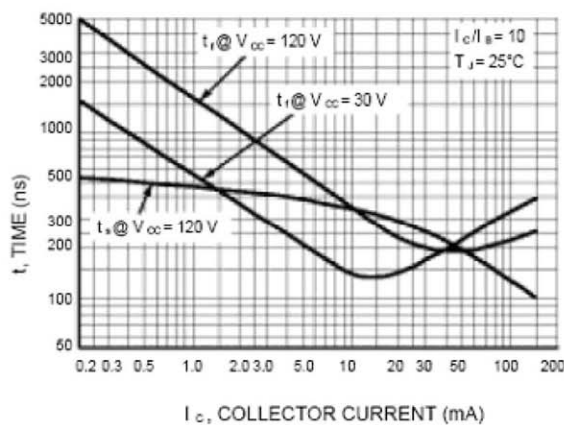
Figure 18. Turn-Off Time
