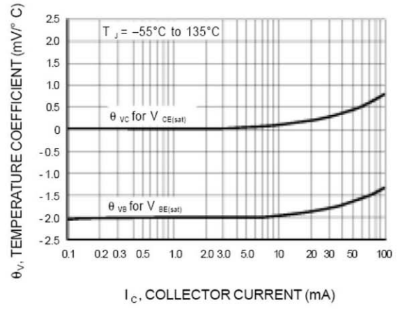
Figure 5. Temperature Coefficients
