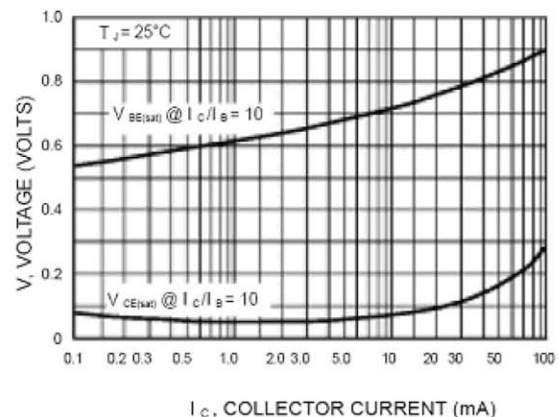
Figure 13. "On" Voltages
