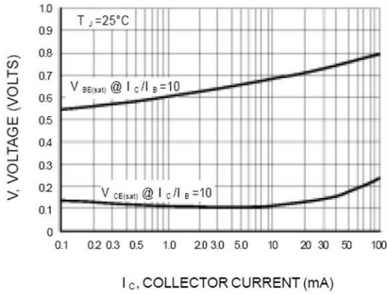
Figure 4. "On" Voltages
