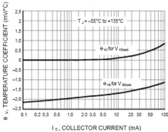
Figure 14. Temperature Coefficients
