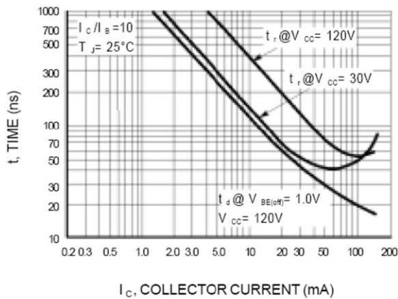
Figure 8. Turn-On Time
