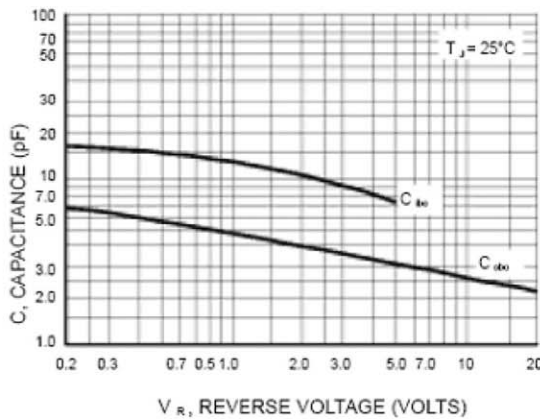
Figure 16. Capacitances Figure
