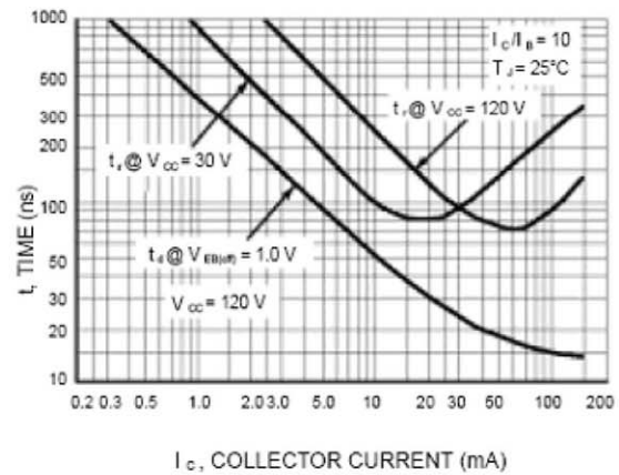
Figure 17. Turn-On Time
