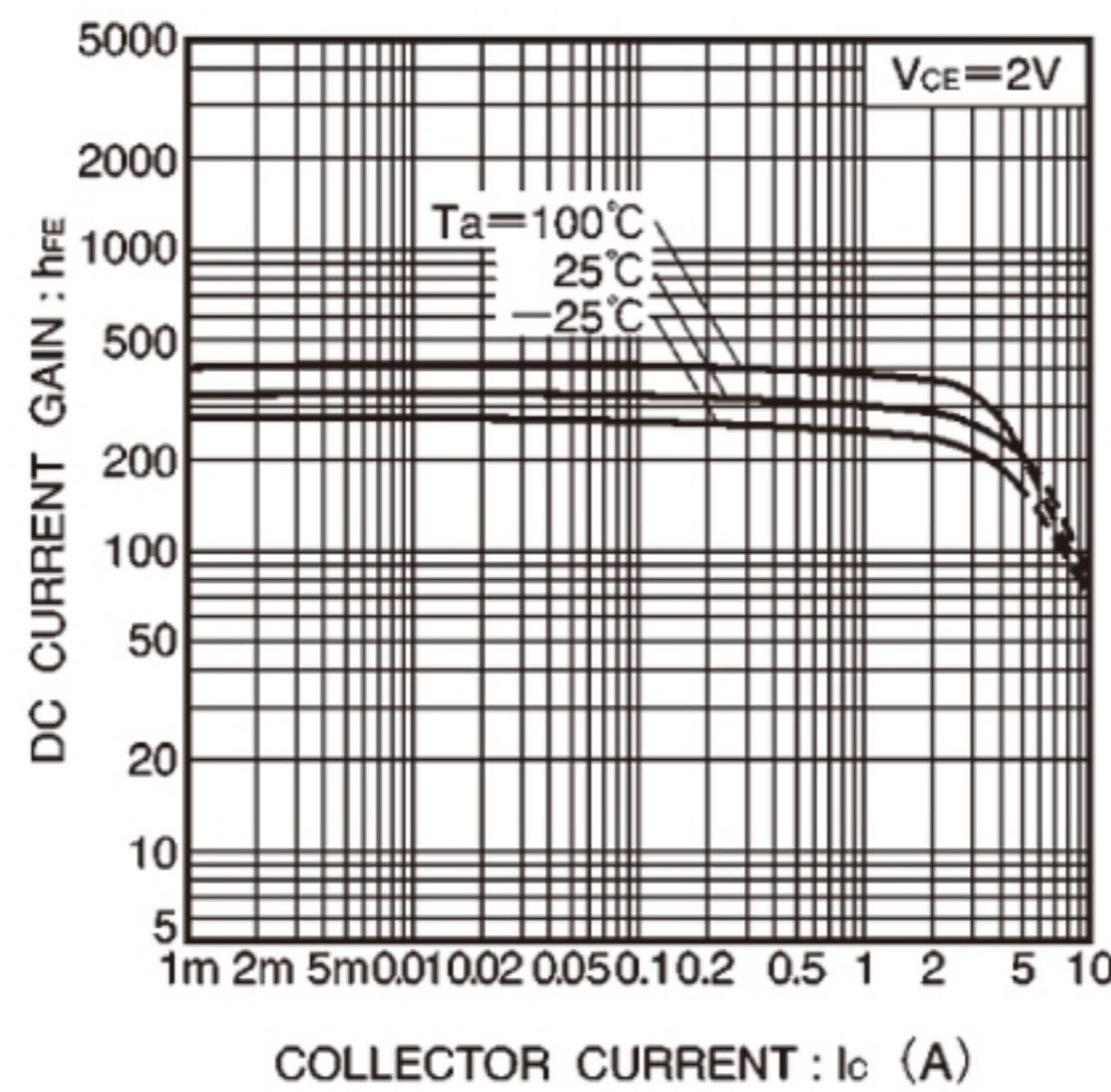
Fig.5 DC current gain vs. collector current ( III )
