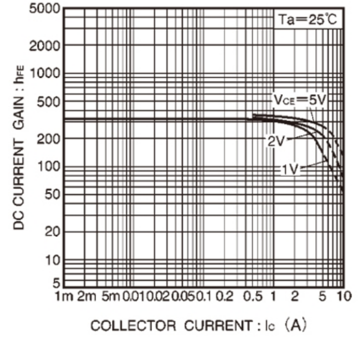
Fig.3 DC current gain vs. collector current ( I )
