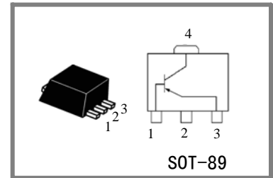
1 Base 2/4 Collector 3 Emitter
