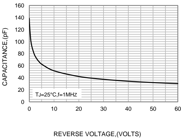
FIG.3-TYPICAL JUNCTION CAPACITANCE
