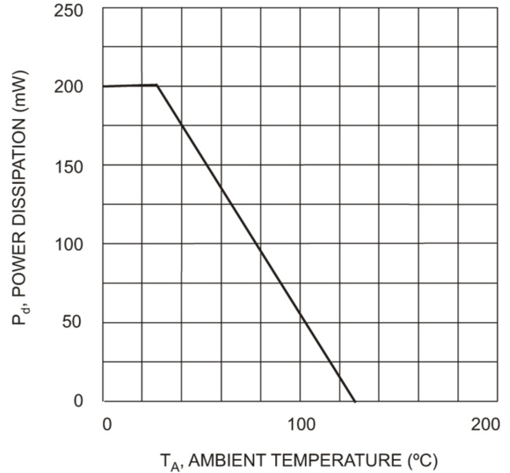
Fig. 4 Power Derating Curve, Total Package
