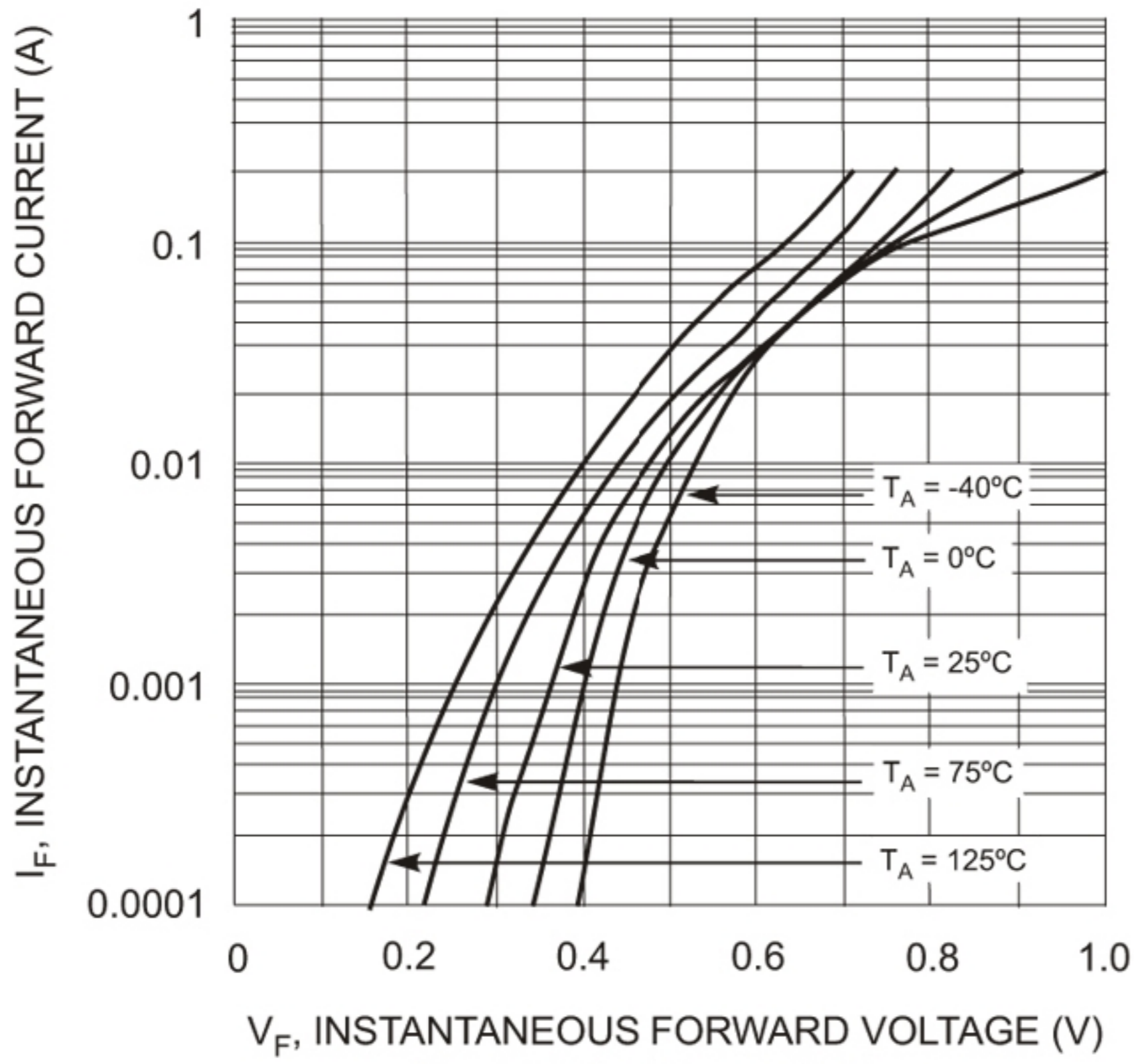
Fig. 1 Typical Forward Voltage
