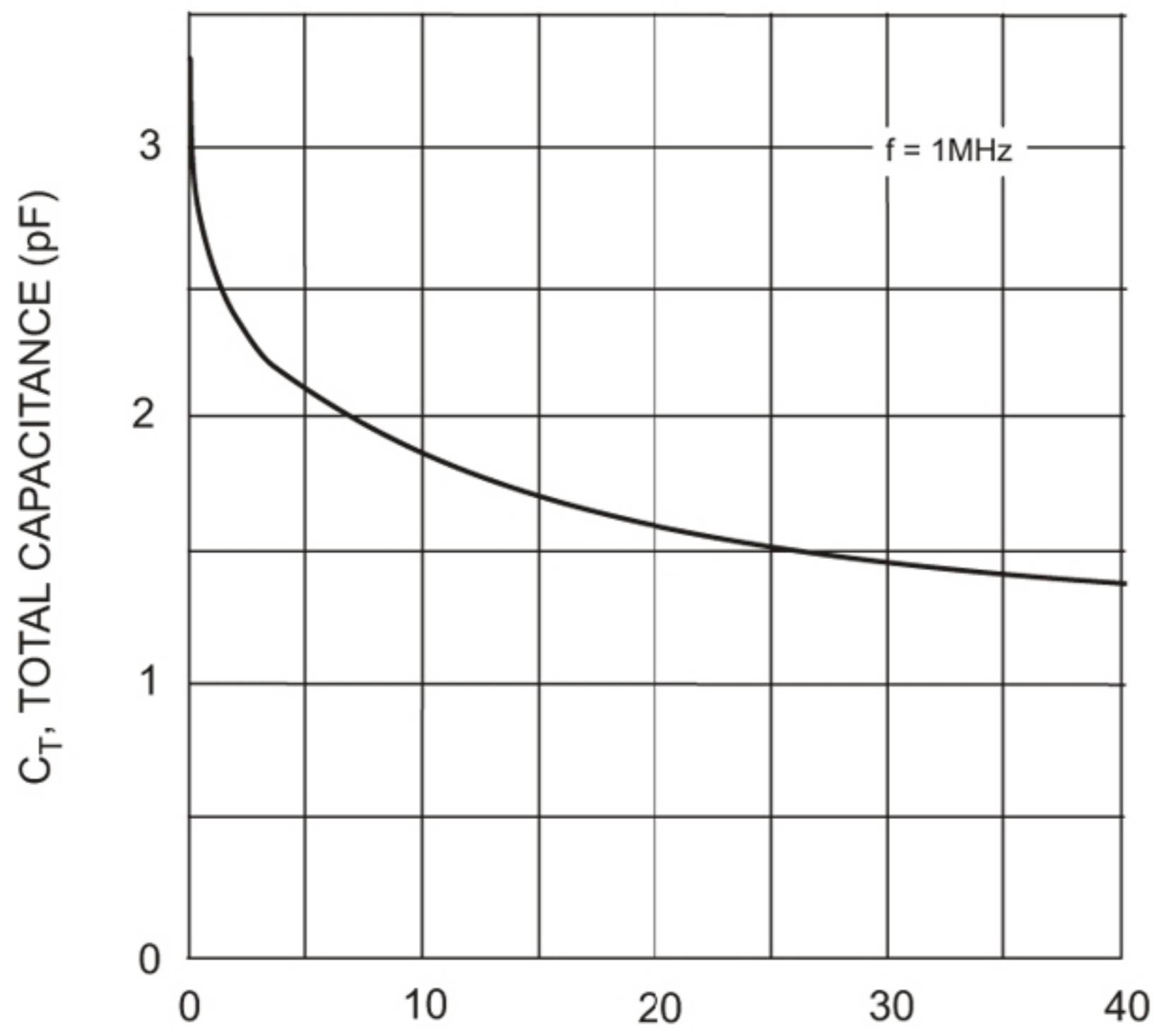
Fig. 3 Typical Capacitance
