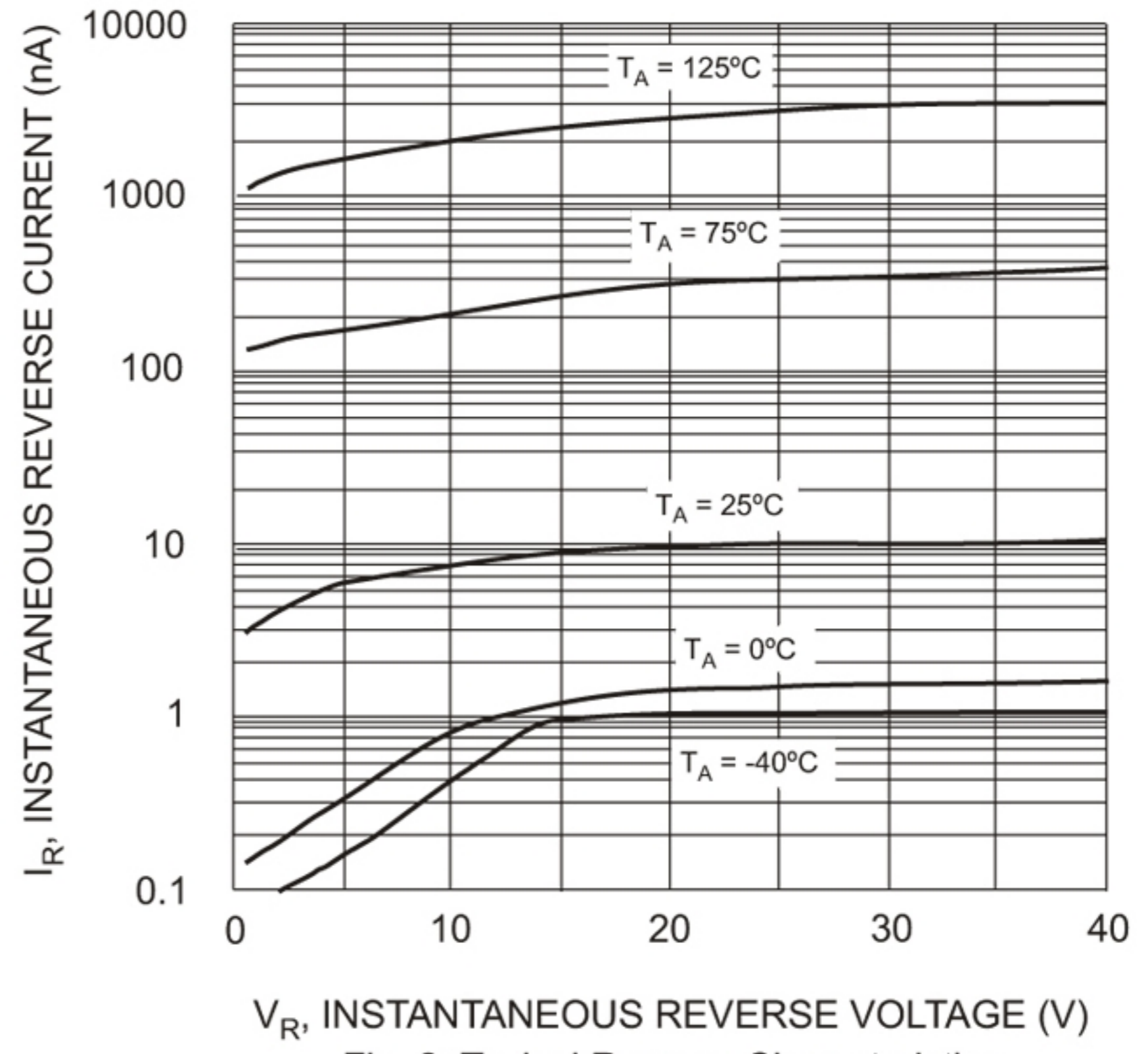
Fig. 2 Typical Reverse Characteristics
